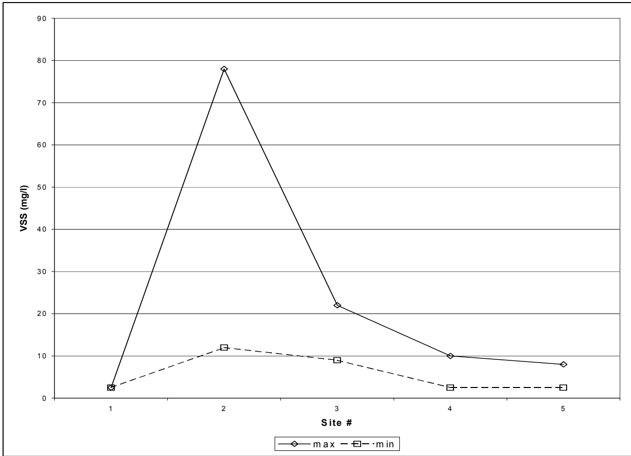
Figure 2: VSS in West Fork Sni-A-Bar from a Stream Survey in July, 2003
