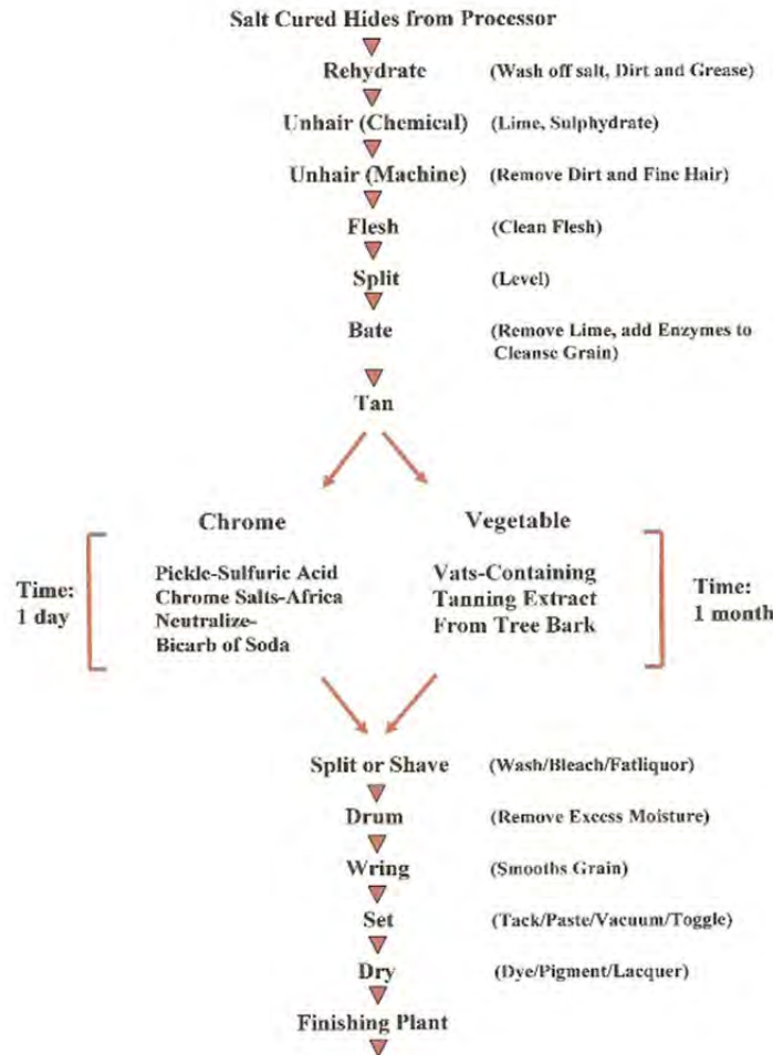
Figure 1, Tanning Process
